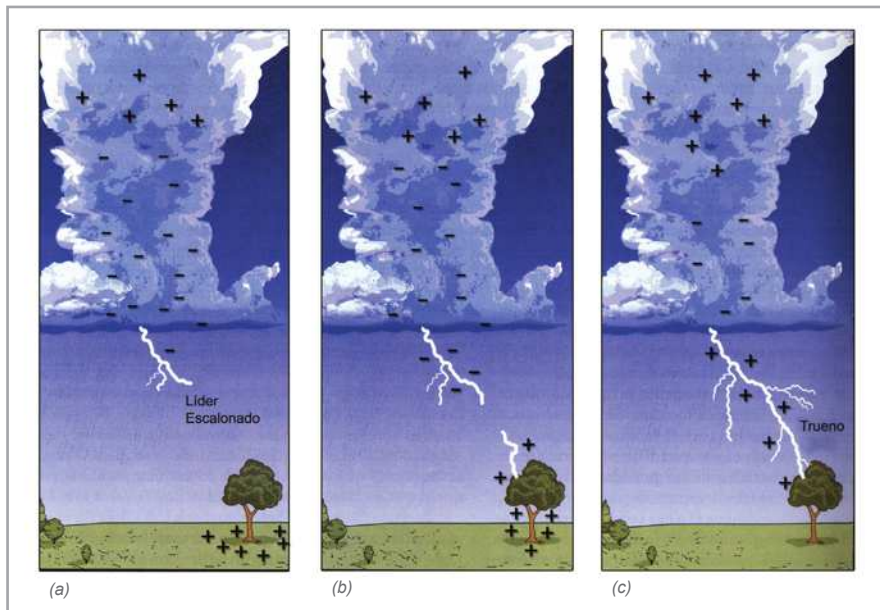
Model for forked lightning. (a) The negative charge concentrated at the bottom of the cloud becomes large enough to overcome the air's resistance and develops a «leader» pointing towards the ground. (b) An upward flow of positive charges from the ground concentrates elevated points. (c) The downward flow of negative charges meets the upward flow of positive charges and a strong electric current known as return stroke carries the positive charges into the cloud.
